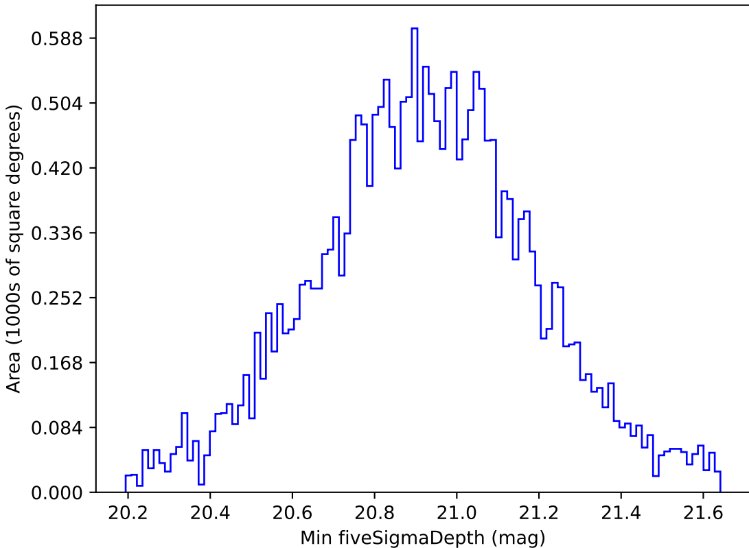
ddf_acor_sf15_lsf30_lsr10_v3.4_10yrs All sky y band: Min fiveSigmaDepth
