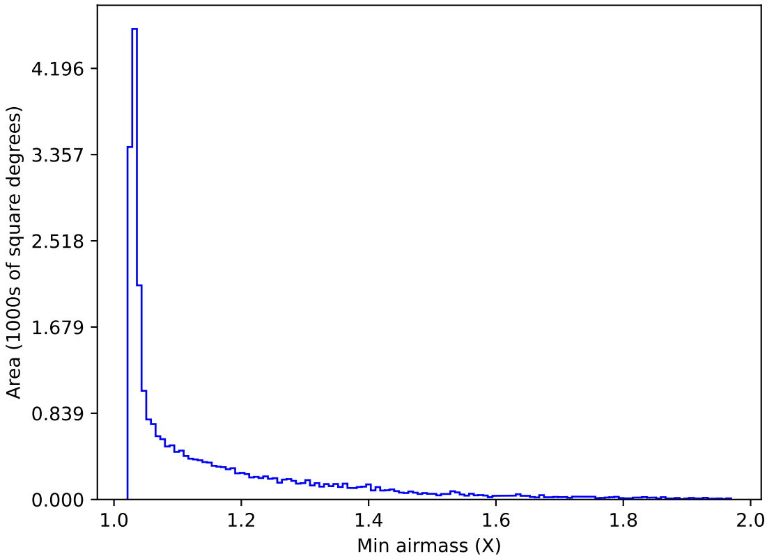
ddf_acor_sf15_lsf30_lsr10_v3.4_10yrs Yr 1 all bands: Min airmass
