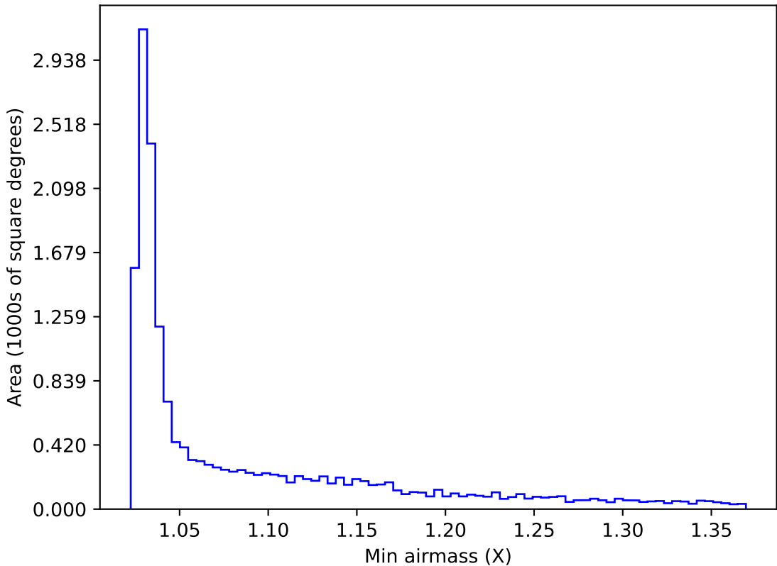
ddf_acor_sf15_lsf30_lsr10_v3.4_10yrs WFD y band: Min airmass
