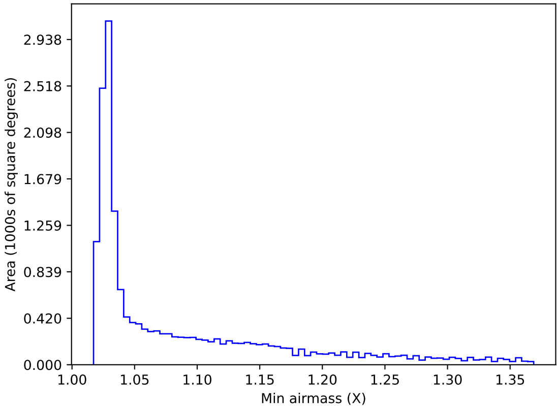
ddf_acor_sf15_lsf30_lsr10_v3.4_10yrs WFD r band: Min airmass
