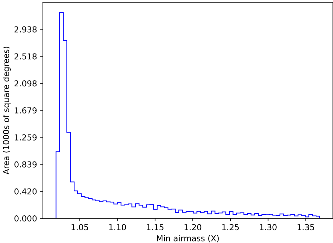
ddf_acor_sf15_lsf30_lsr10_v3.4_10yrs WFD i band: Min airmass
