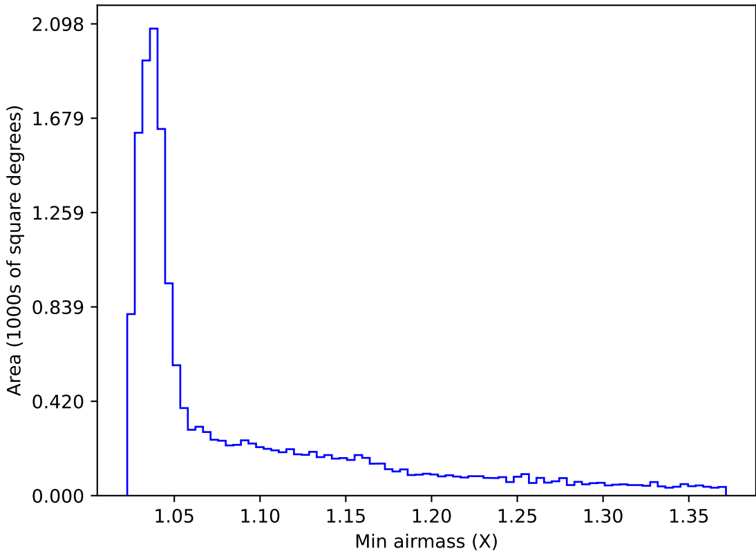
ddf_acor_sf15_lsf30_lsr10_v3.4_10yrs WFD g band: Min airmass
