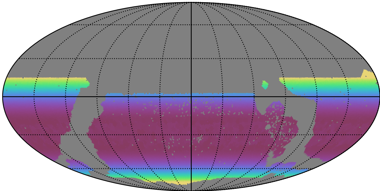
ddf_acor_sf15_lsf30_lsr10_v3.4_10yrs WFD all bands: Min airmass
