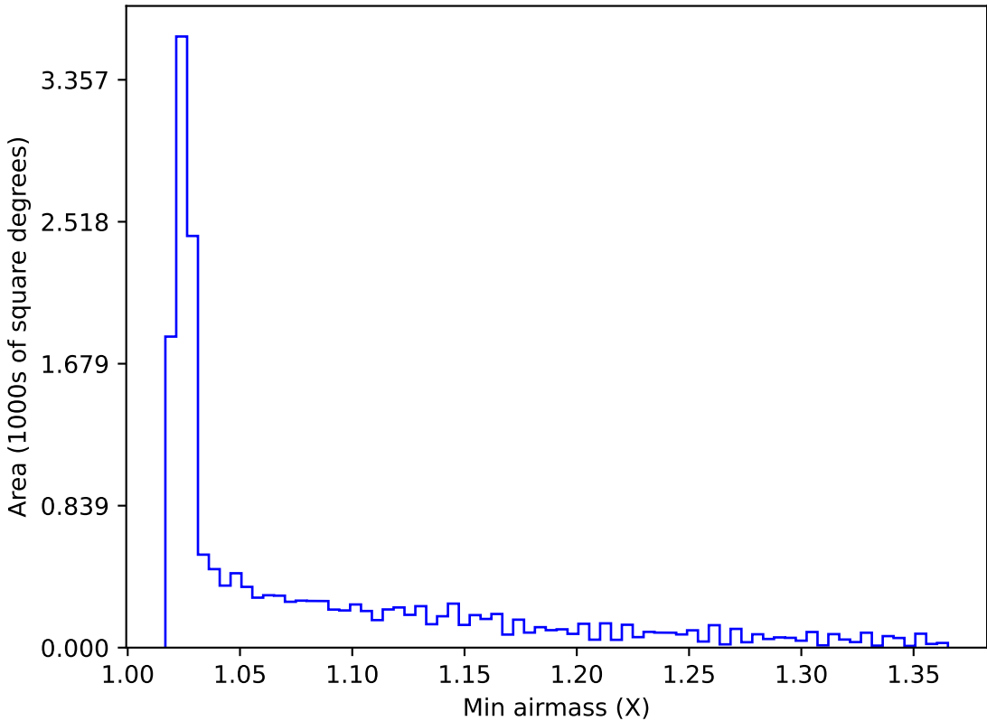
ddf_acor_sf15_lsf30_lsr10_v3.4_10yrs WFD all bands: Min airmass
