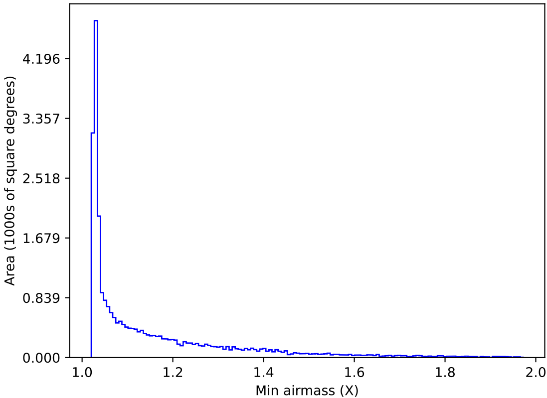
ddf_acor_sf15_lsf30_lsr10_v3.4_10yrs All sky z band: Min airmass
