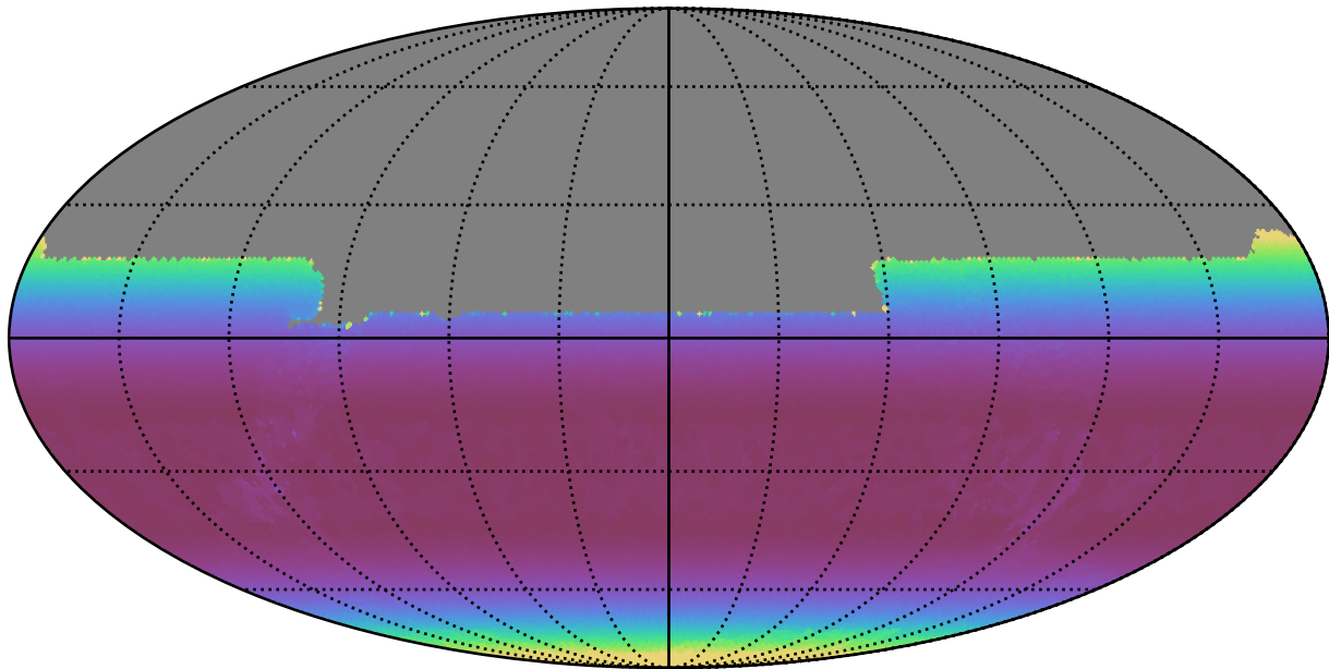
ddf_acor_sf15_lsf30_lsr10_v3.4_10yrs All sky y band: Min airmass
