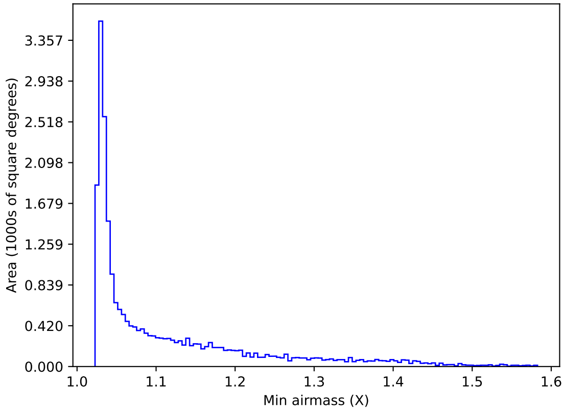
ddf_acor_sf15_lsf30_lsr10_v3.4_10yrs All sky y band: Min airmass
