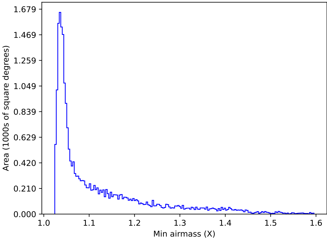
ddf_acor_sf15_lsf30_lsr10_v3.4_10yrs All sky u band: Min airmass
