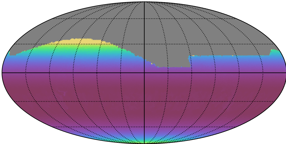
ddf_acor_sf15_lsf30_lsr10_v3.4_10yrs All sky r band: Min airmass
