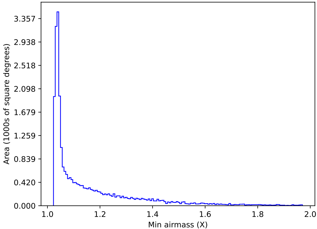
ddf_acor_sf15_lsf30_lsr10_v3.4_10yrs All sky g band: Min airmass
