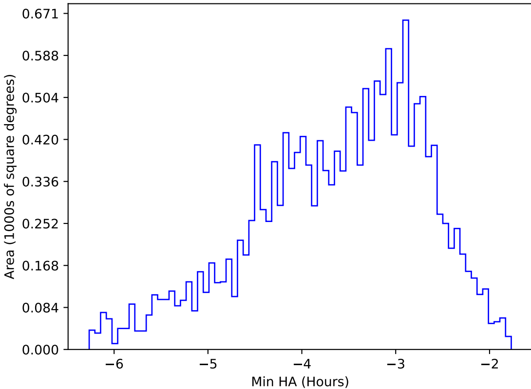
ddf_acor_sf15_lsf30_lsr10_v3.4_10yrs WFD y band: Min HA
