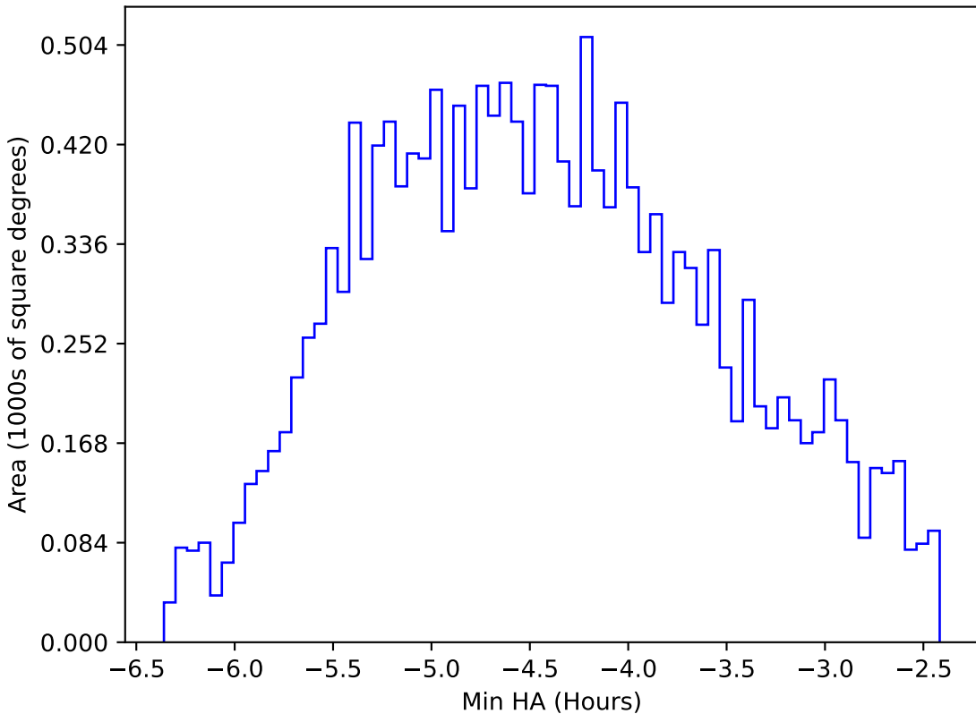
ddf_acor_sf15_lsf30_lsr10_v3.4_10yrs WFD r band: Min HA
