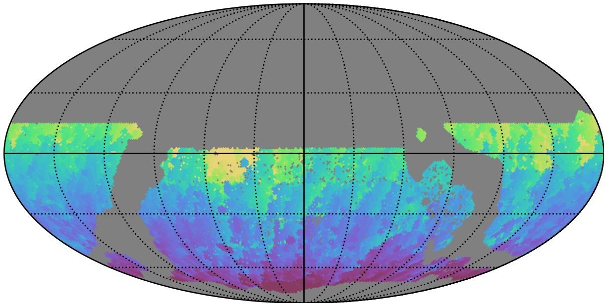
ddf_acor_sf15_lsf30_lsr10_v3.4_10yrs WFD g band: Min HA
