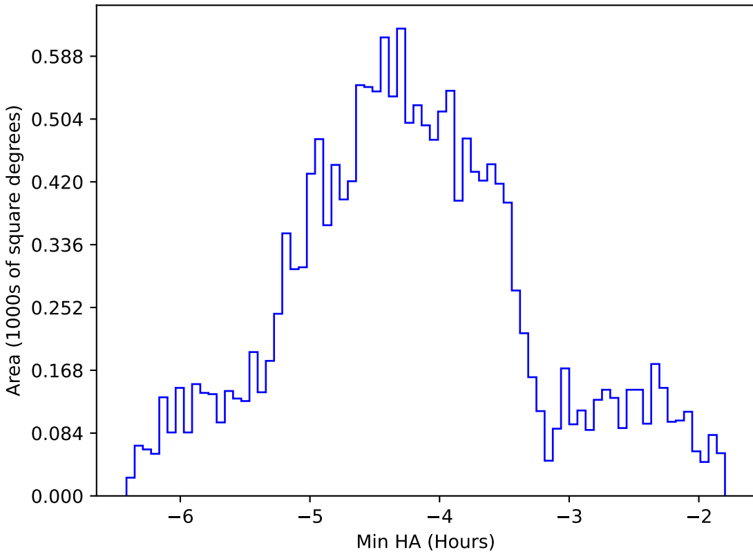
ddf_acor_sf15_lsf30_lsr10_v3.4_10yrs WFD g band: Min HA
