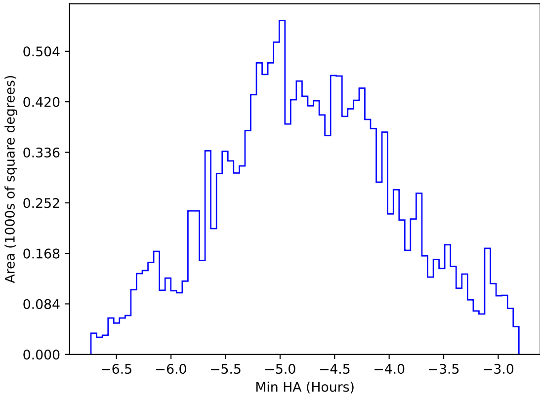
ddf_acor_sf15_ls30_lsr10_v3.4_10yrs WFD all bands: Min HA
