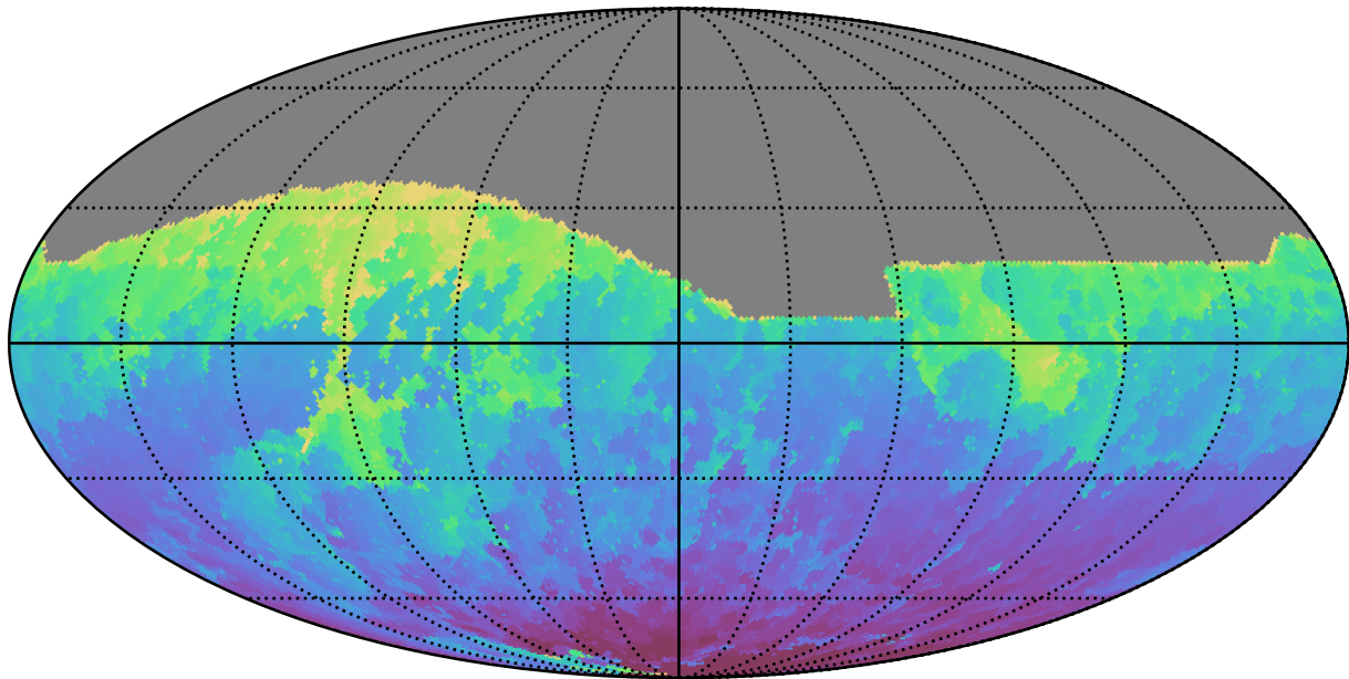
ddf_acor_sf15_lsf30_lsr10_v3.4_10yrs All sky z band: Min HA
