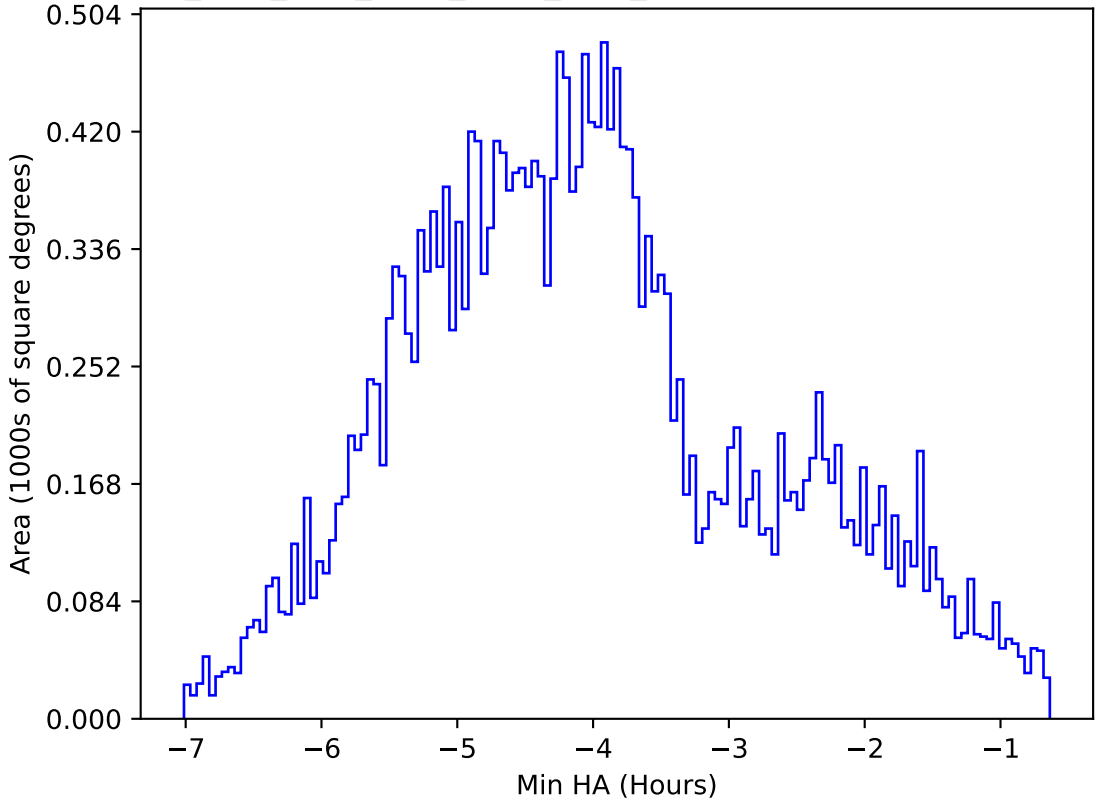
ddf_acor_sf15_lsf30_lsr10_v3.4_10yrs All sky z band: Min HA
