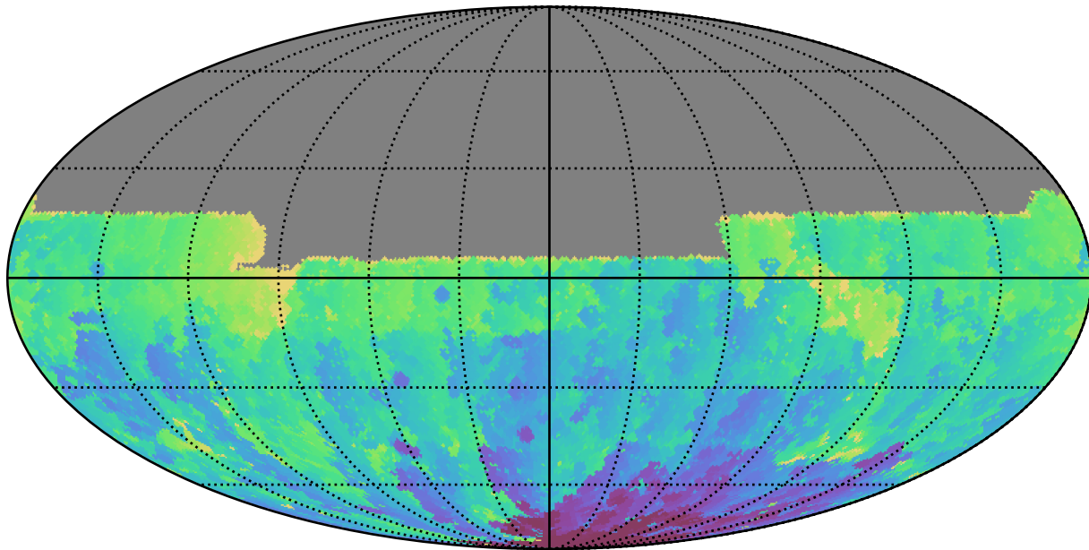
ddf_acor_sf15_lsf30_lsr10_v3.4_10yrs All sky u band: Min HA
