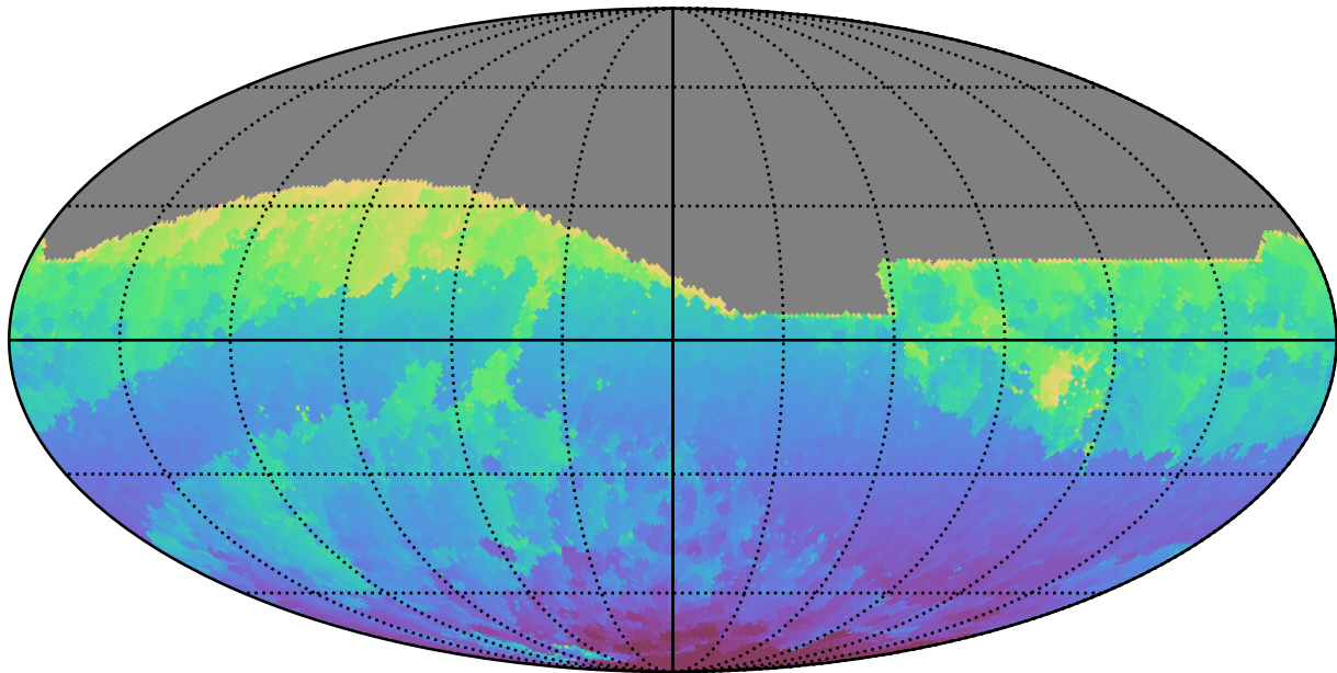
ddf_acor_sf15_lsf30_lsr10_v3.4_10yrs All sky r band: Min HA
