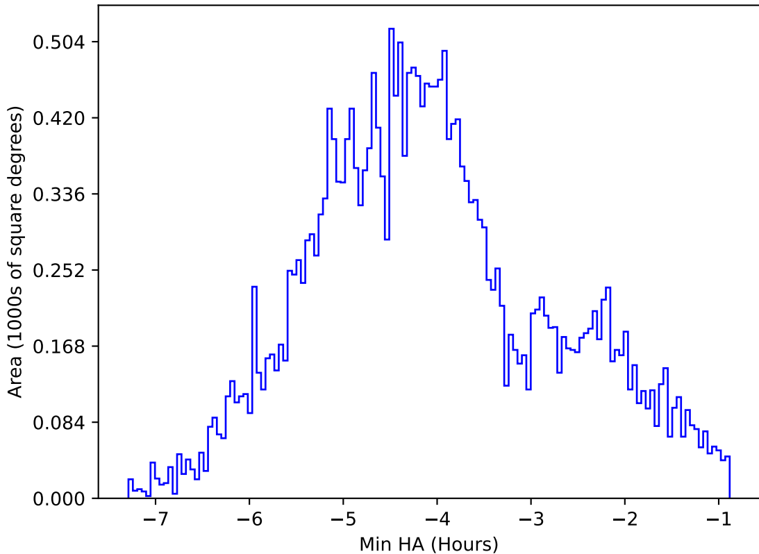
ddf_acor_sf15_ls30_lsr10_v3.4_10yrs All sky i band: Min HA
