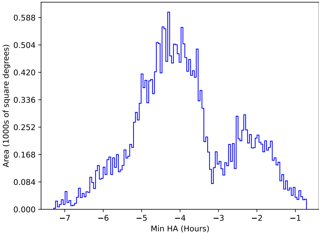
ddf_acor_sf15_lsf30_lsr10_v3.4_10yrs All sky g band: Min HA
