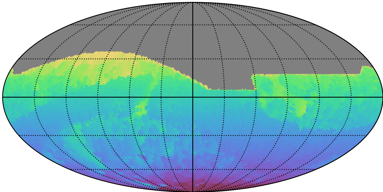
ddf_acor_sf15_lsf30_lsr10_v3.4_10yrs All sky all bands: Min HA
