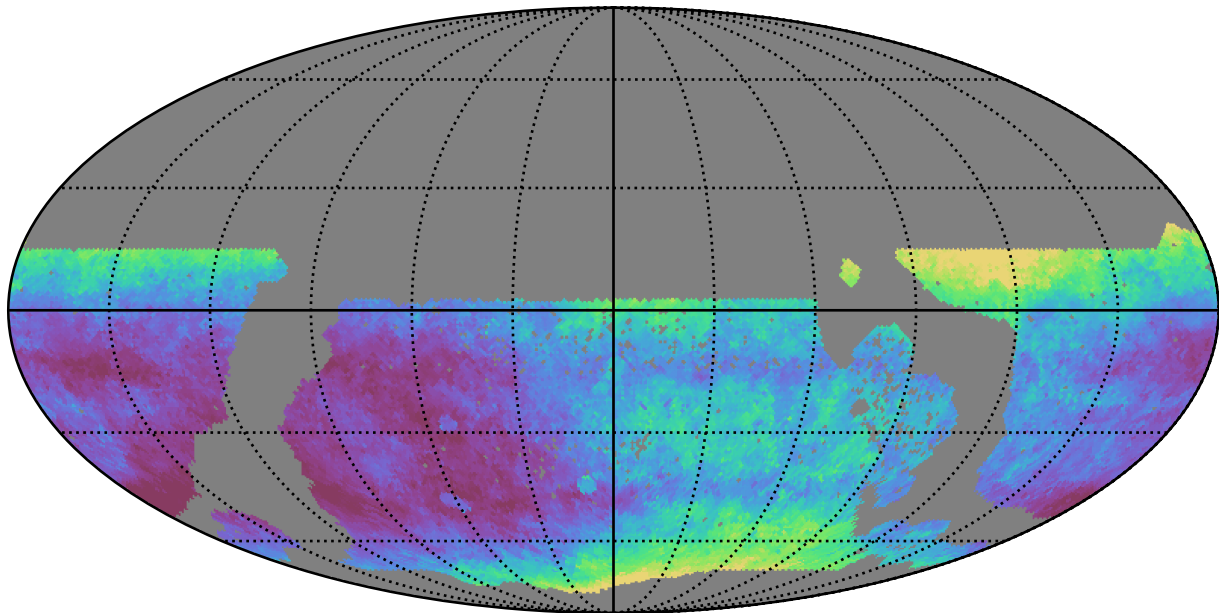
ddf_acor_sf15_lsf30_lsr10_v3.4_10yrs WFD i band: Median seeingEff
