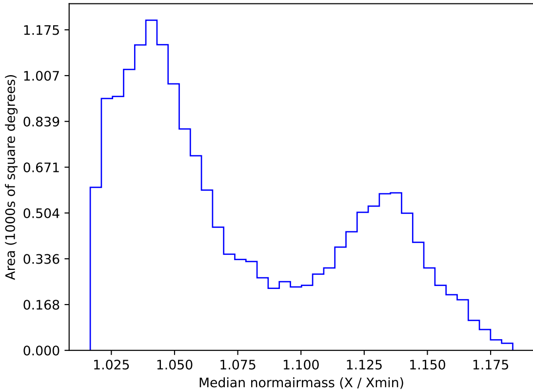
ddf_acor_sf15_lsf30_lsr10_v3.4_10yrs WFD r band: Median normairmass
