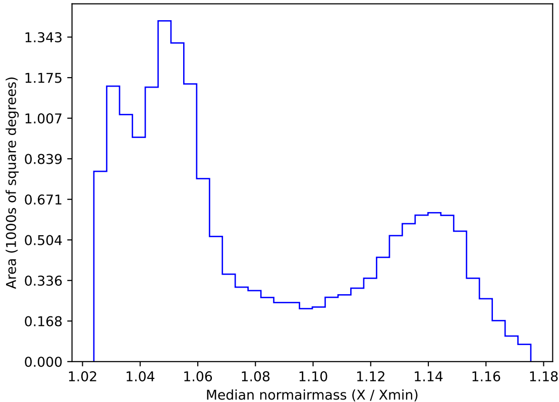
ddf_acor_sf15_lsf30_lsr10_v3.4_10yrs WFD all bands: Median normairmass
