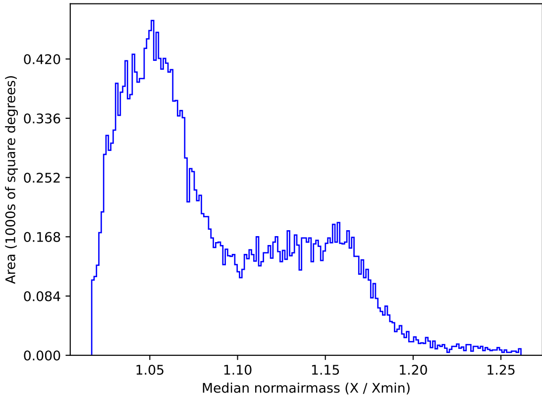
ddf_acor_sf15_ls30_lsr10_v3.4_10yrs All sky z band: Median normairmass
