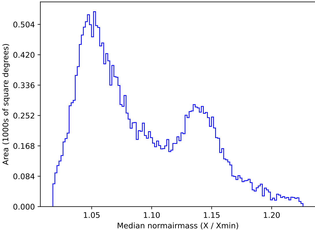
ddf_acor_sf15_lsf30_lsr10_v3.4_10yrs All sky y band: Median normairmass
