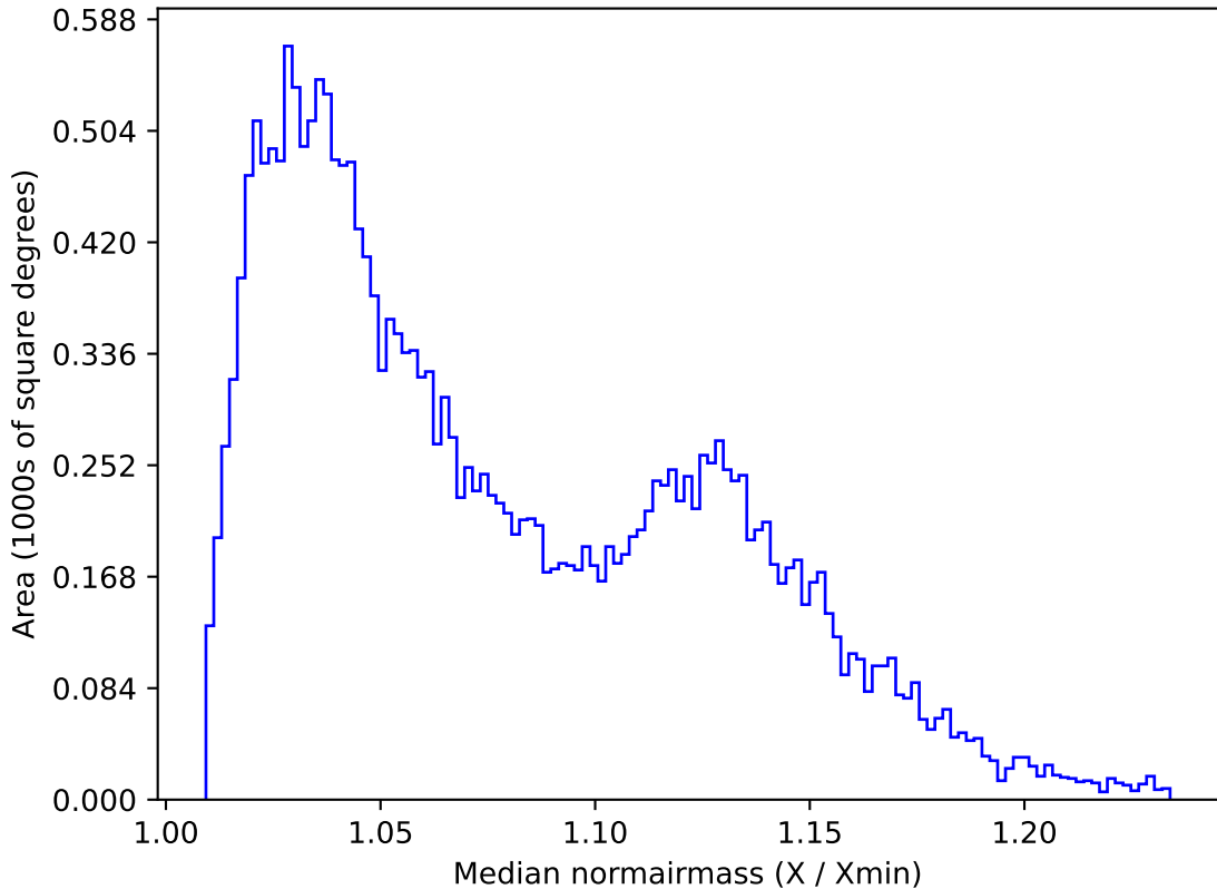
ddf_acor_sf15_lsf30_lsr10_v3.4_10yrs All sky u band: Median normairmass
