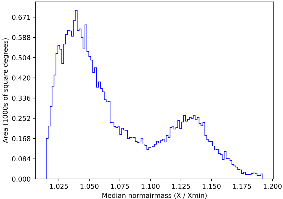
ddf_acor_sf15_lsf30_lsr10_v3.4_10yrs All sky r band: Median normairmass
