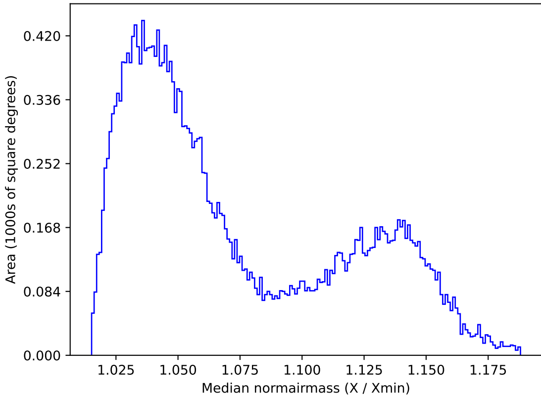
ddf_acor_sf15_lsf30_lsr10_v3.4_10yrs All sky i band: Median normairmass
