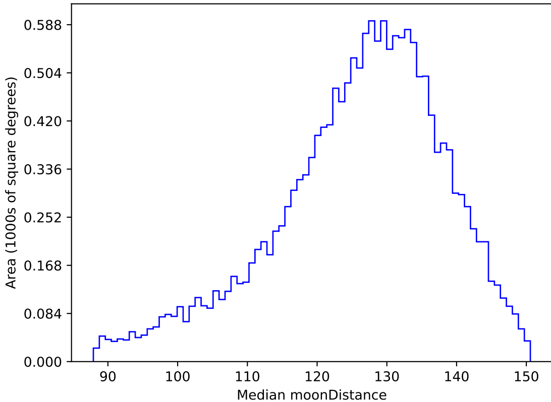
ddf_acor_sf15_lsf30_lsr10_v3.4_10yrs WFD u band: Median moonDistance
