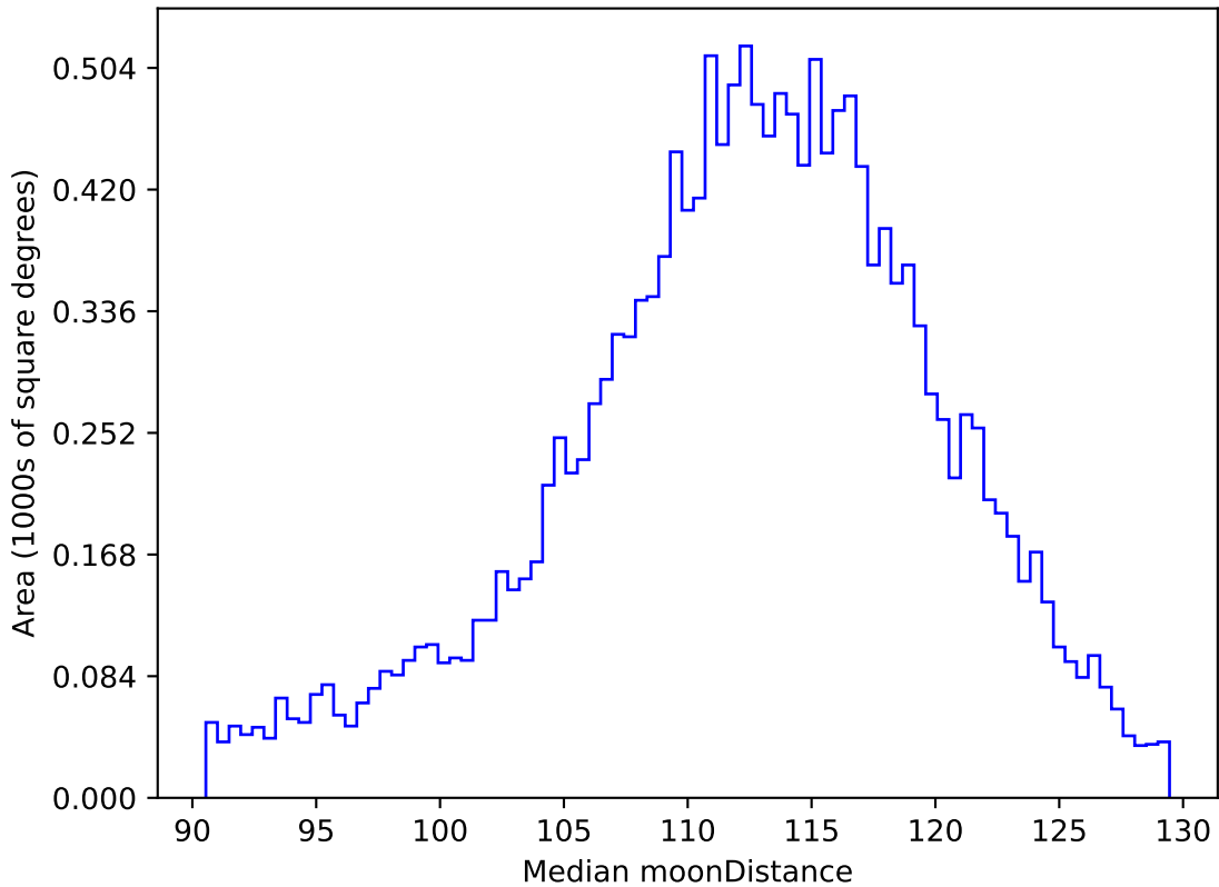
ddf_acor_sf15_lsf30_lsr10_v3.4_10yrs WFD r band: Median moonDistance
