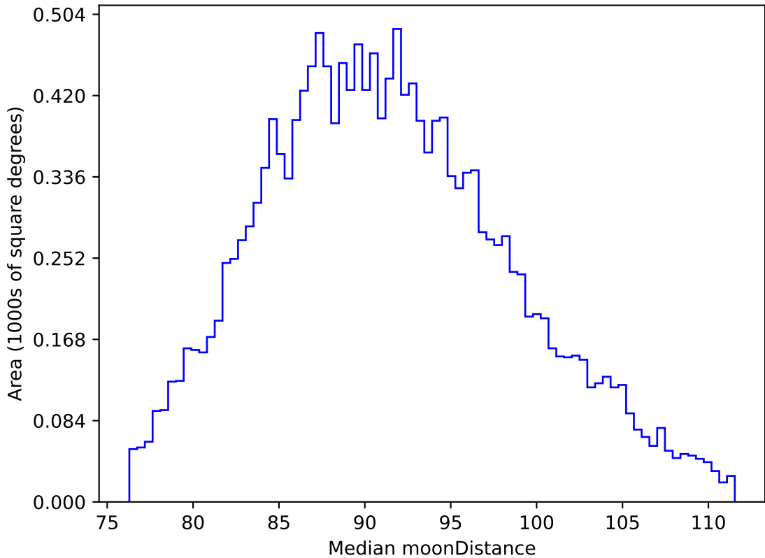
ddf_acor_sf15_lsf30_lsr10_v3.4_10yrs WFD i band: Median moonDistance
