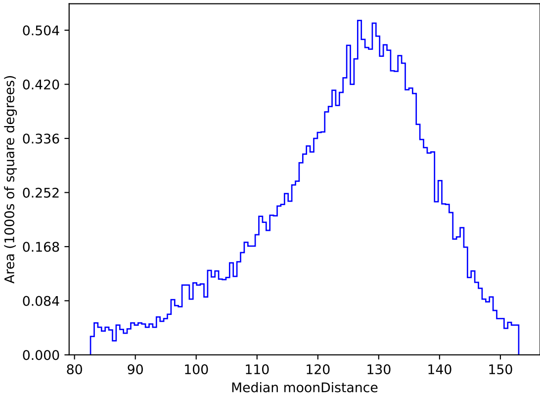
ddf_acor_sf15_lsf30_lsr10_v3.4_10yrs All sky u band: Median moonDistance
