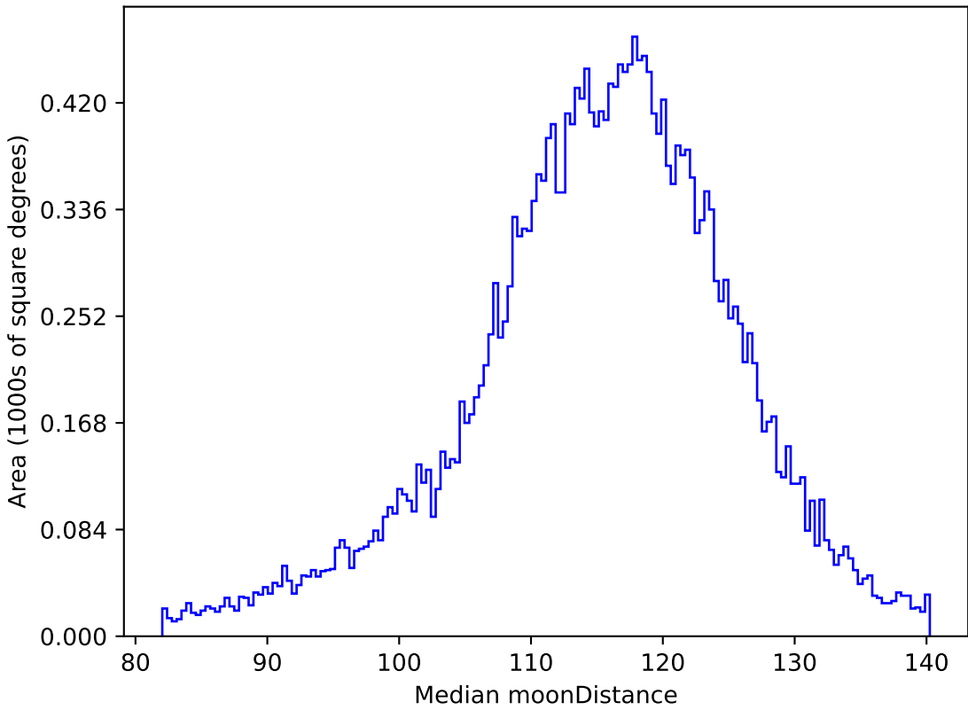
ddf_acor_sf15_lsf30_lsr10_v3.4_10yrs All sky g band: Median moonDistance
