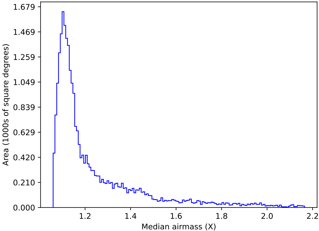
ddf_acor_sf15_lsf30_lsr10_v3.4_10yrs Yr 1 i band: Median airmass
