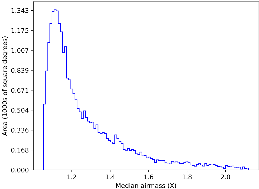
ddf_acor_sf15_lsf30_lsr10_v3.4_10yrs Yr 1 g band: Median airmass
