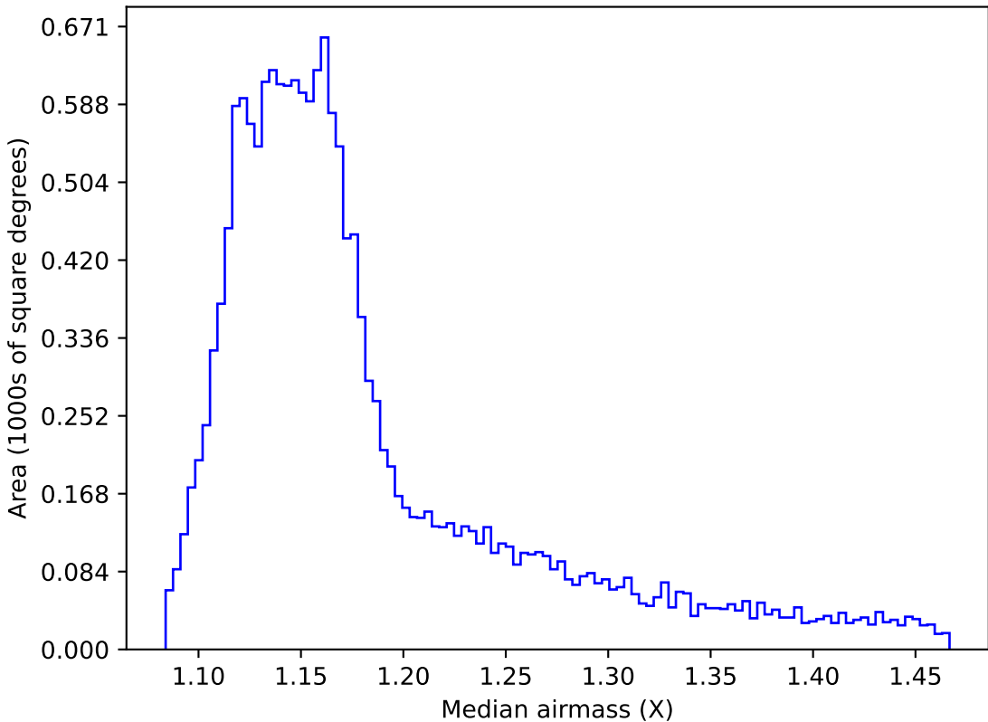
ddf_acor_sf15_lsf30_lsr10_v3.4_10yrs WFD z band: Median airmass
