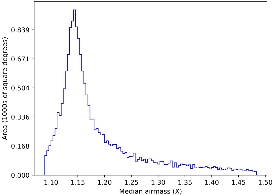
ddf_acor_sf15_ls30_lsr10_v3.4_10yrs WFD y band: Median airmass
