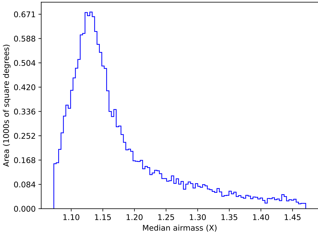
ddf_acor_sf15_lsf30_lsr10_v3.4_10yrs WFD u band: Median airmass
