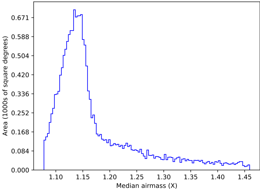
ddf_acor_sf15_lsf30_lsr10_v3.4_10yrs WFD i band: Median airmass
