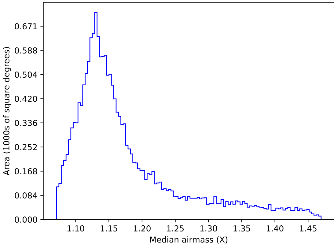
ddf_acor_sf15_lsf30_lsr10_v3.4_10yrs WFD g band: Median airmass
