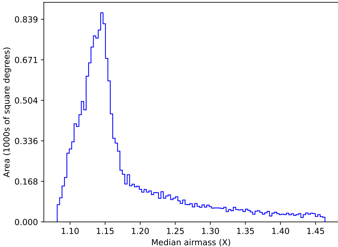
ddf_acor_sf15_lsf30_lsr10_v3.4_10yrs WFD all bands: Median airmass
