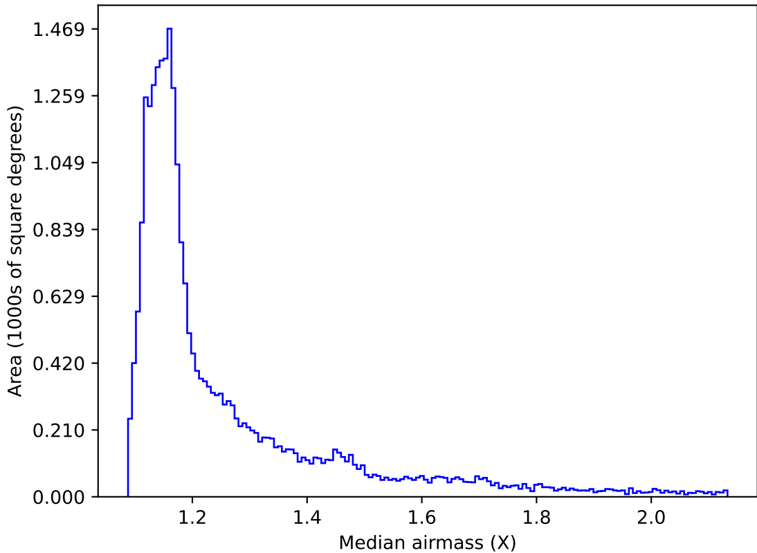
ddf_acor_sf15_lsf30_lsr10_v3.4_10yrs All sky z band: Median airmass
