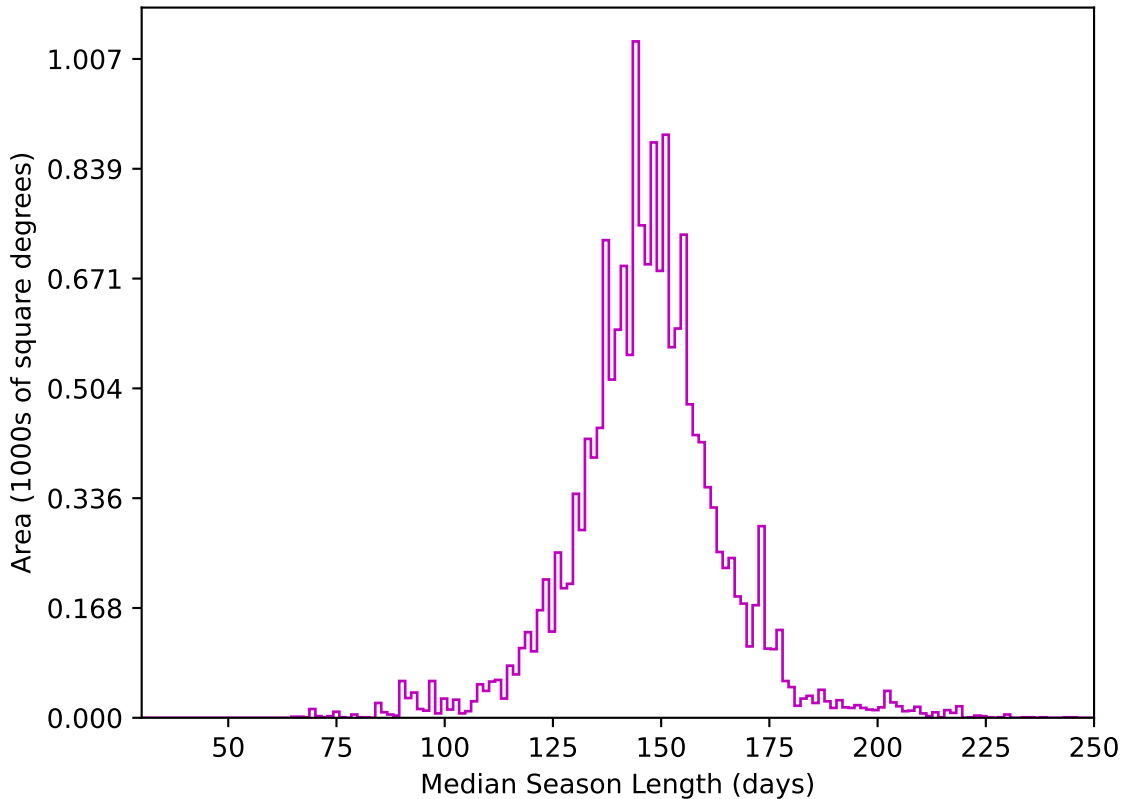
ddf_acor_sf15_lsf30_lsr10_v3.4_10yrs WFD z band: Median Season Length
