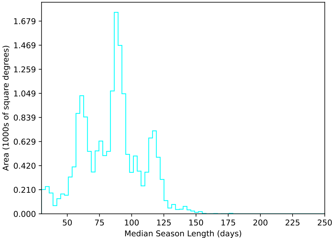
ddf_acor_sf15_ls30_lsr10_v3.4_10yrs WFD u band: Median Season Length
